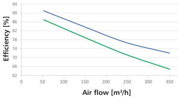
Performance curve Heat (—) and moisture recovery (—) HRU-SlimAIR-350E
