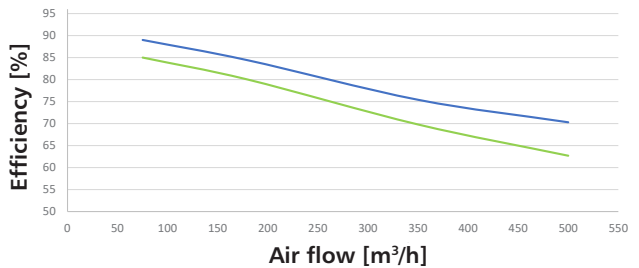
Performance curve Heat (—) and moisture recovery (—) HRU-SlimAIR-500E
