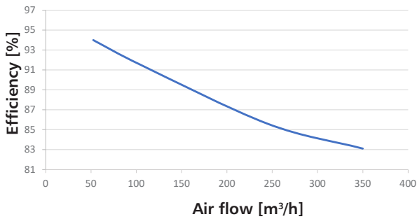
Performance curve HRU-SlimAIR-350
