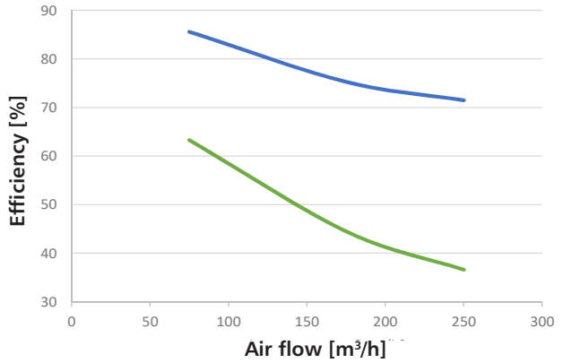
Performance curve Heat (—) and moisture recovery (—) HRU-SlimAIR-250E-H
