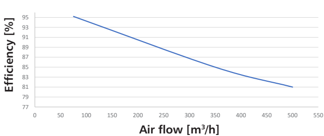
Performance curve HRU-SlimAIR-500
